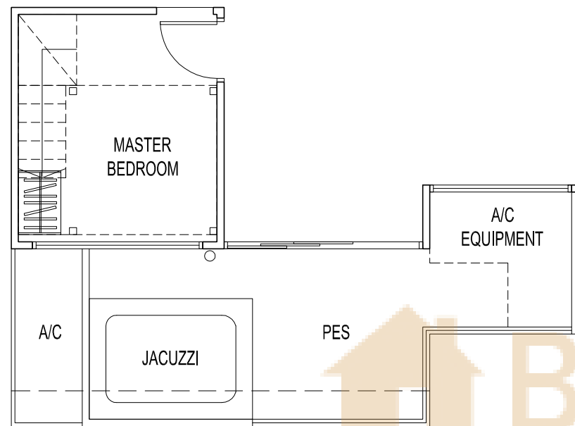
1ST STOREY PART PLAN
