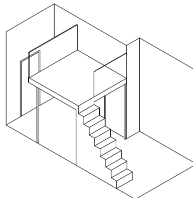
LOFT LAYOUT ISOMETRIC VIEW
