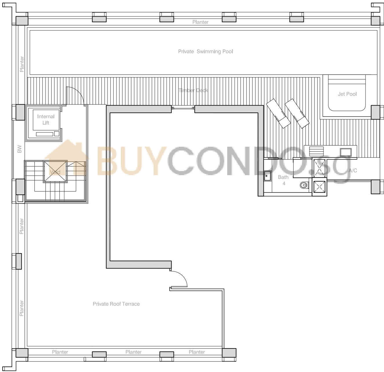
ROOF TERRACE
