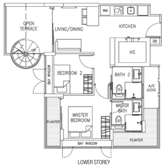
LOWER STOREY
