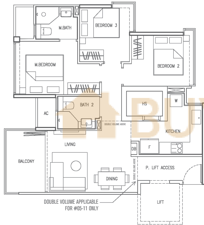
TYPE C3 / C3-PH
