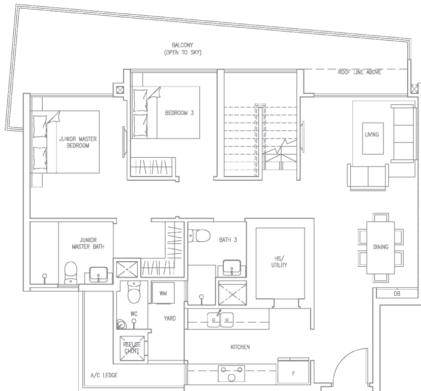
LOWER LEVEL
