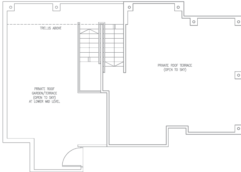
ROOF LEVEL
