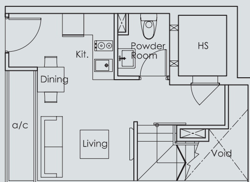
LOWER LEVEL
