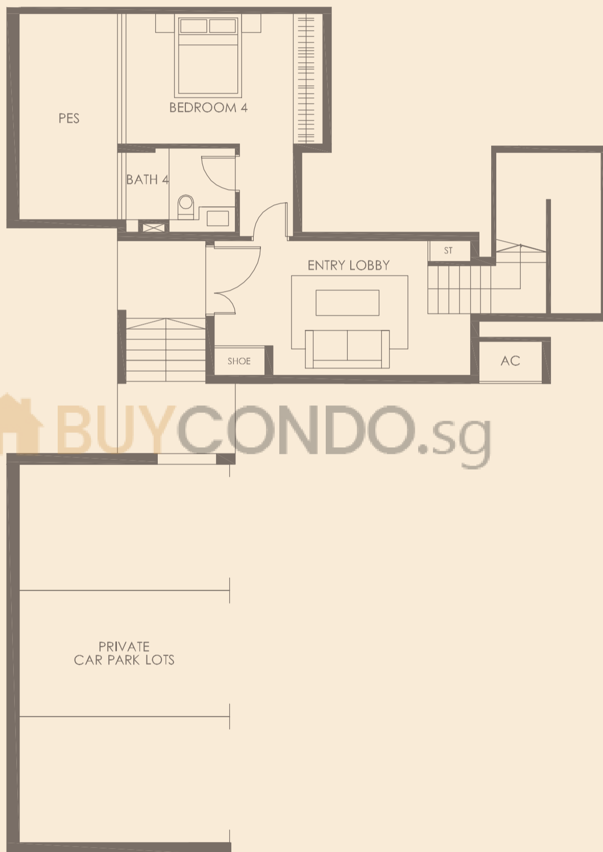
BASEMENT PLAN
