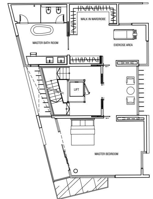
Level 3 Plan
