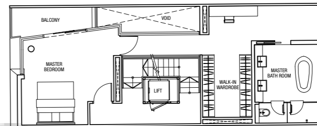
Level 3 Plan
