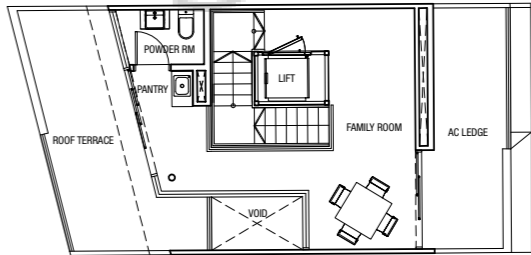
Attic Plan
