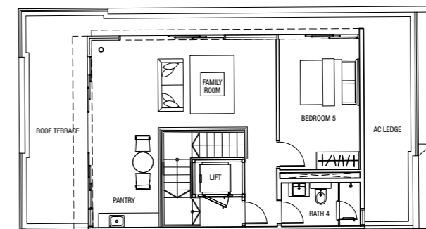
Attic Plan
