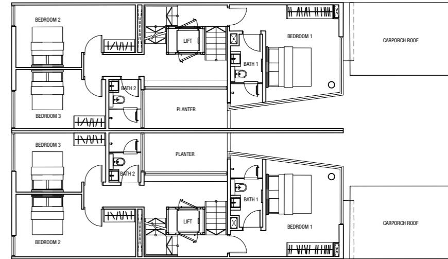
Level 2 Plan
