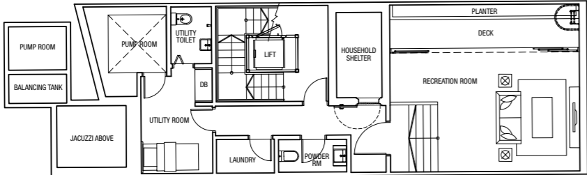
Basement Plan
