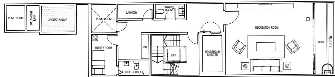
Basement Plan
