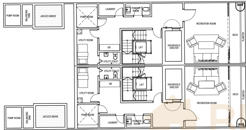
Basement Plan
