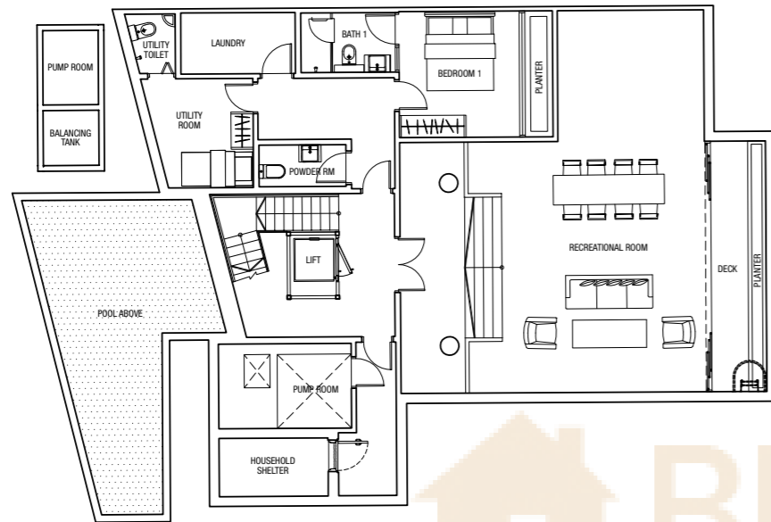
Level 1 Plan
