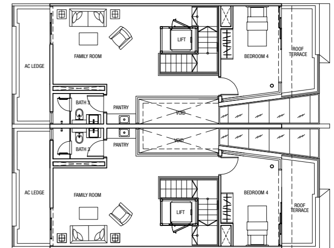
Attic Plan
