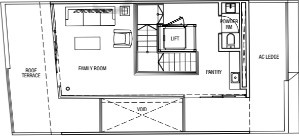
Attic Plan
