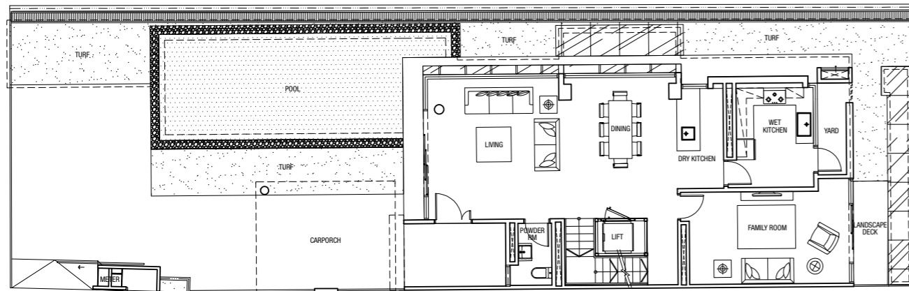
Level 1 Plan
