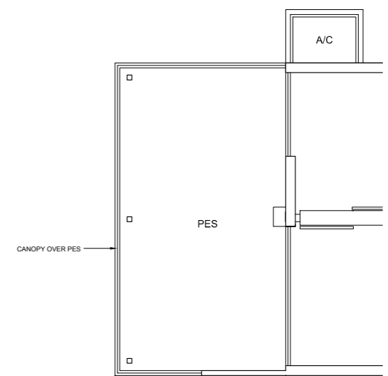
TYPE A2(p) 72 sqm / 775 sqft #07-03
