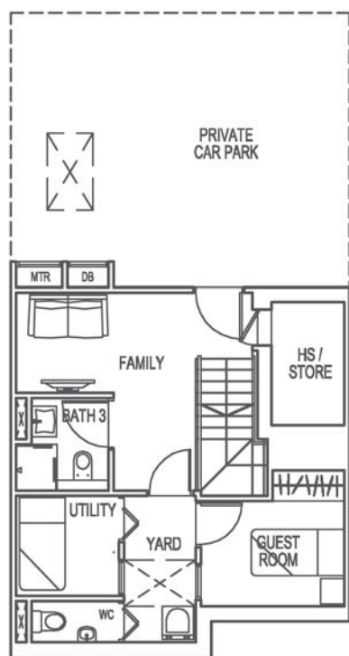
BASEMENT
