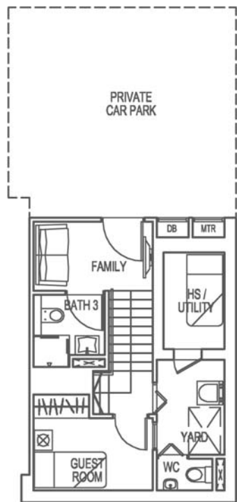
BASEMENT
