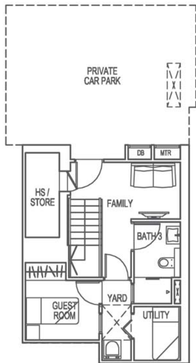
BASEMENT
