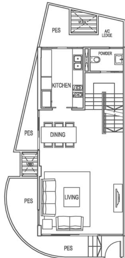
1ST STOREY
