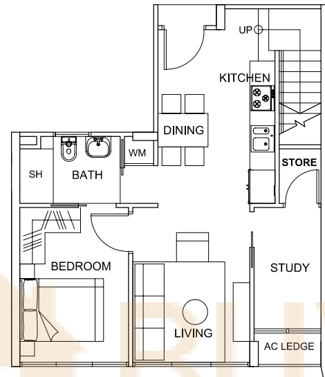
5TH STOREY PLAN
