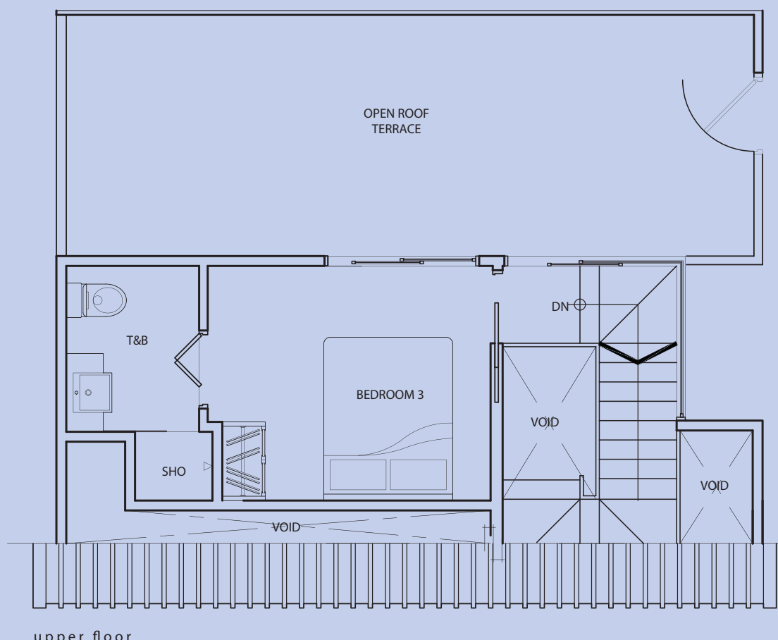
upper floor
