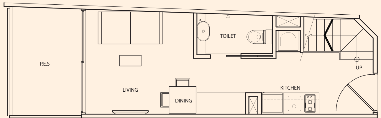
lower floor
