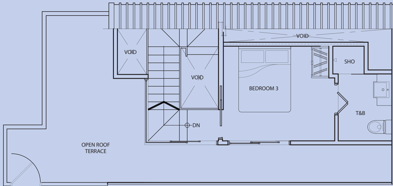
upper floor
