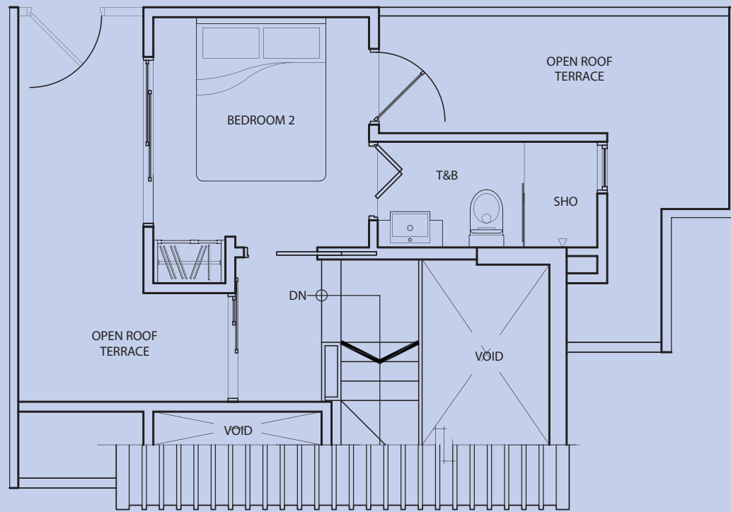
upper floor
