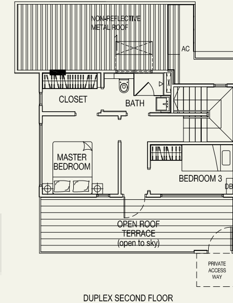
DUPLEX SECOND FLOOR
