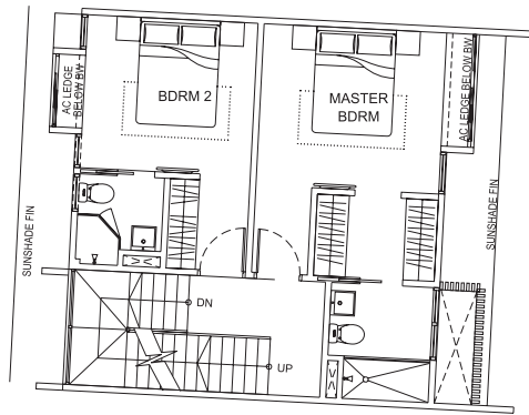
2nd flr
