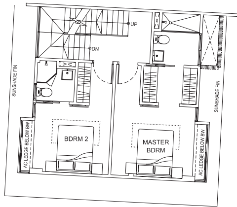
2nd flr
