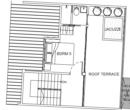
attic
