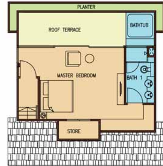
ATTIC PLAN
