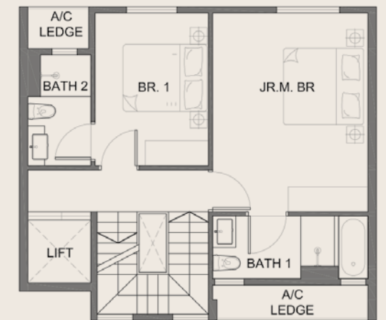
2ND STOREY
