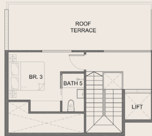
ATTIC STOREY
