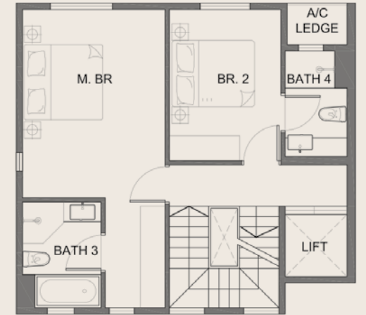
3RD STOREY
