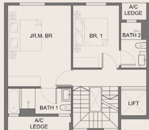
2ND STOREY
