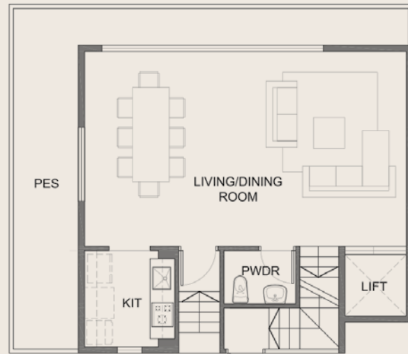
1ST STOREY
