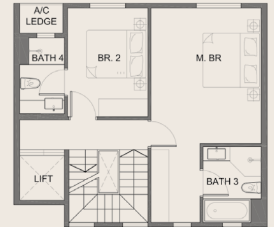
3RD STOREY
