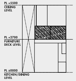
SECTION VIEW
