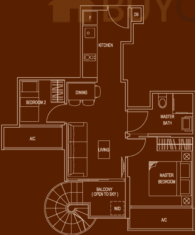
LOWER STOREY
