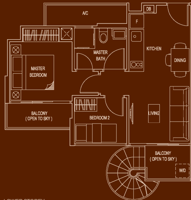
LOWER STOREY
