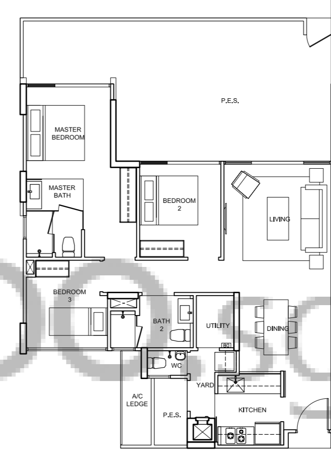
TYPE C1a-pes-01 130 sqm/ 1,402 sq ft 86, Elias Road 100, Elias Road # 01 - 18 # 01 - 19 # 01 - 62
