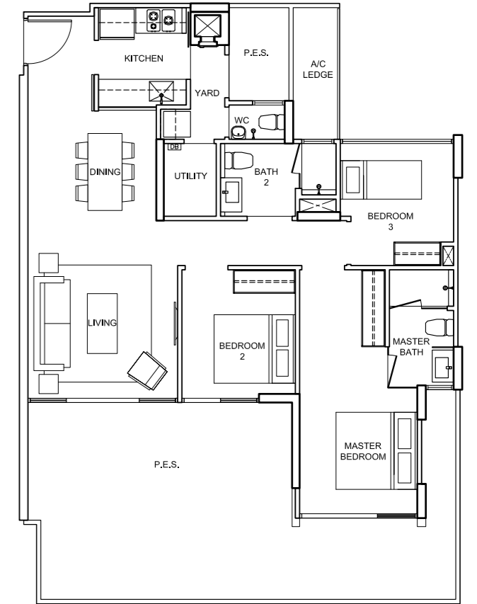
TYPE C4-pes 130 sqm/ 1,402 sq ft 80, Elias Road # 01 - 03
