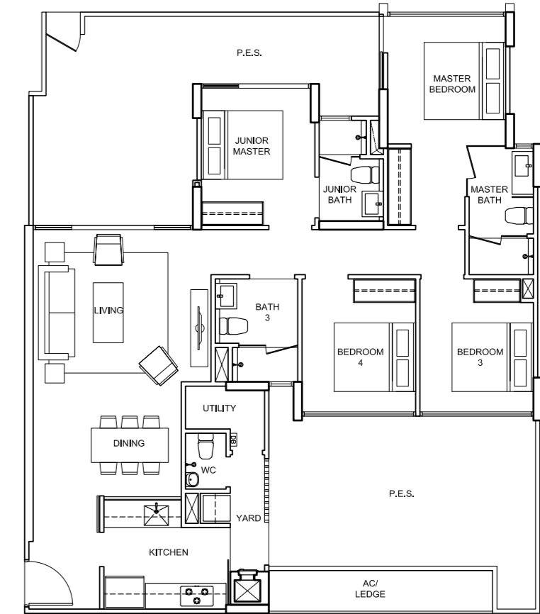
TYPE D3-pes-02 161 sqm/ 1,735 sq ft 90, Elias Road # 01 - 30 94, Elias Road # 01 - 43
