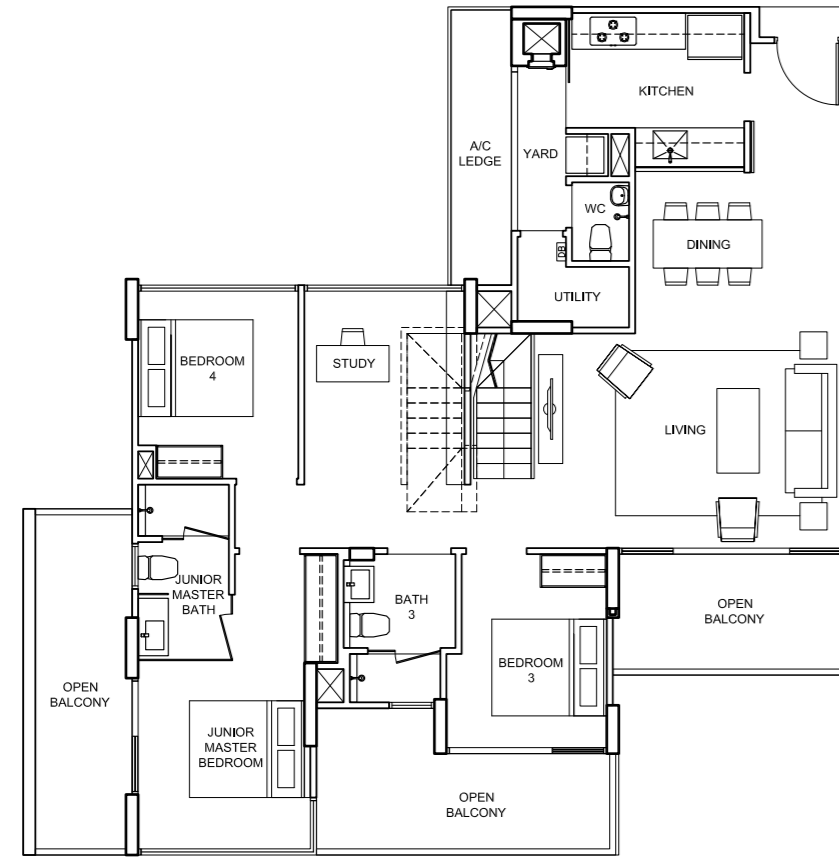
LOWER LEVEL TYPE D1-ph 199 sqm/ 2,145 sq ft 88, Elias Road 94, Elias Road # 05 - 27 # 05 - 45
