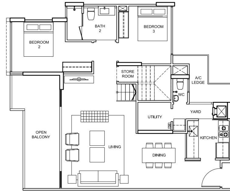
LOWER LEVEL TYPE C2a-ph 162 sqm/ 1,746 sq ft 84, Elias Road # 05 - 12
