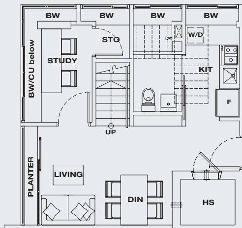
Lower penthouse
