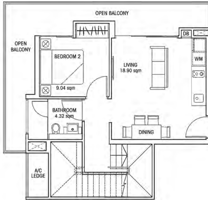
LOWER STOREY
