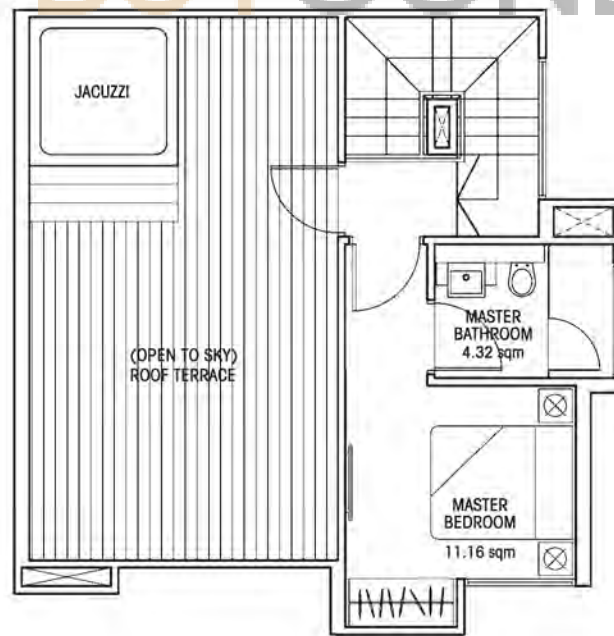
UPPER STOREY
