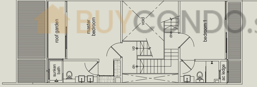
2nd storey
