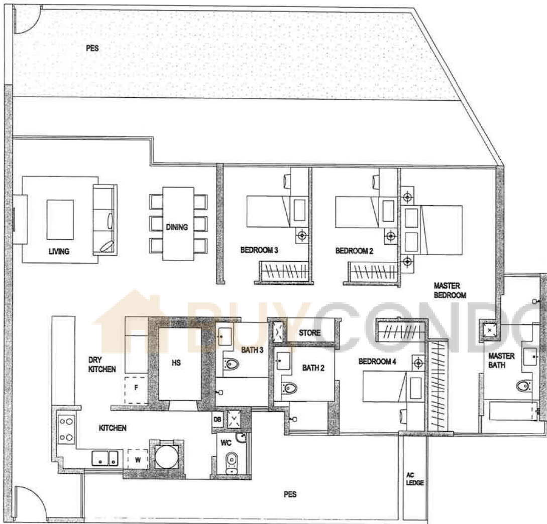
TYPE G2(P5) : 4-BEDROOM — sq m/ —sq ft #01-36
