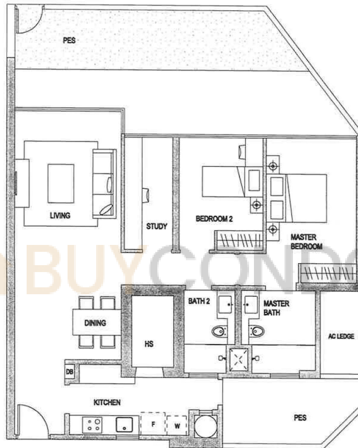
TYPE C2a(P6) : 2-BEDROOM + STUDY — sq m/ —sq ft #01-58 MIRROR IMAGE #01-59
