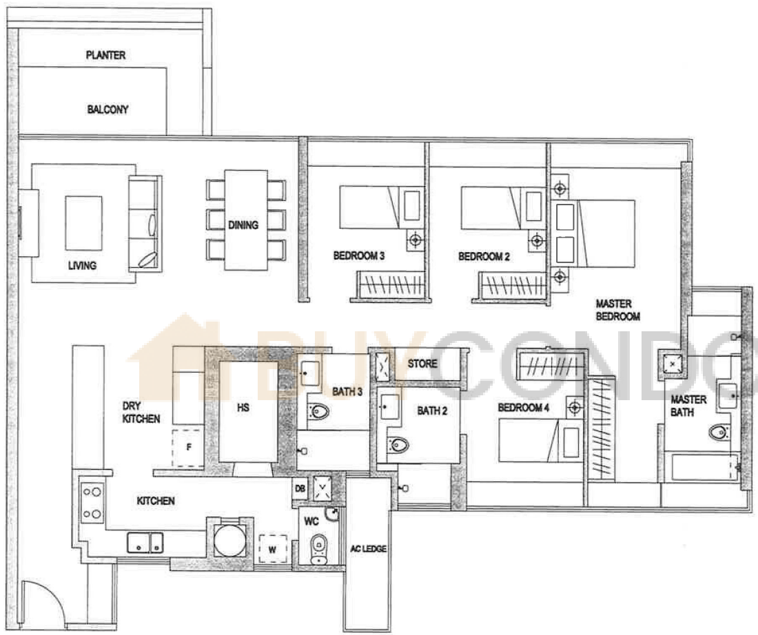
TYPE G2 : 4-BEDROOM — sq m/ —sq ft #02-36 to #14-36 MIRROR IMAGE #02-35 to #14-35, #02-39 to #14-39
