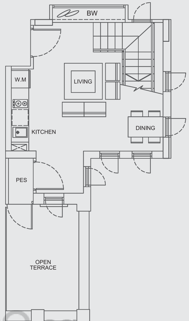
Lower Storey
