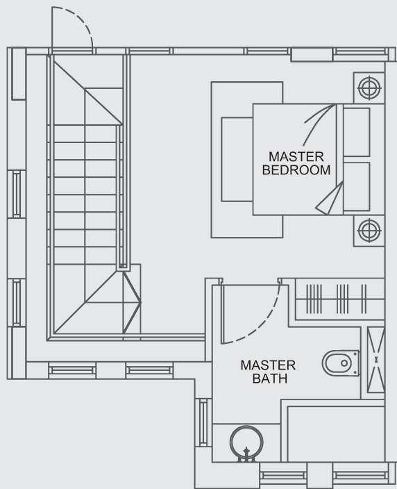
Upper Storey
