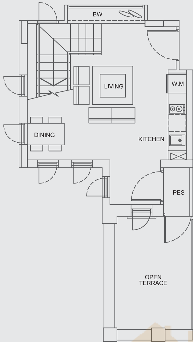
Lower Storey
