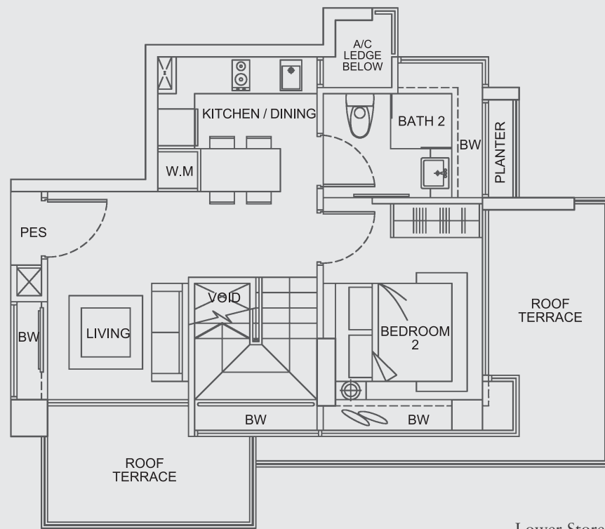
Lower Storey
