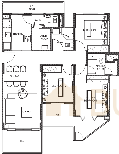
3 Deluxe (3 Bedroom) Type: C4G (mirror-image of C2) (1st storey) Area: 99 sqm #01-28 15 Bartley Road, Singapore 539766
