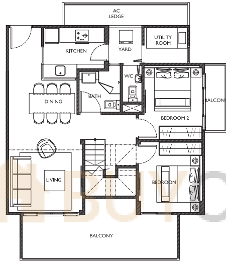
Lower Storey
