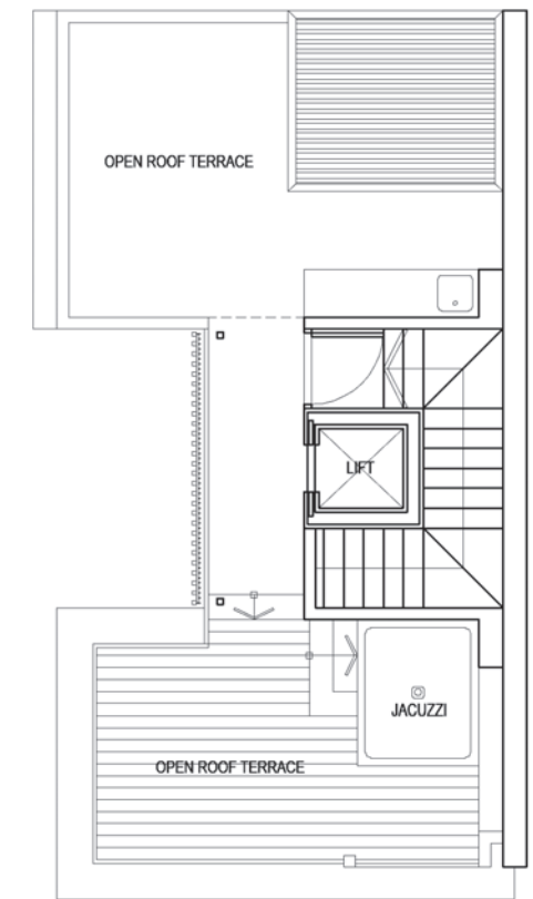
ROOF TERRACE PLAN
