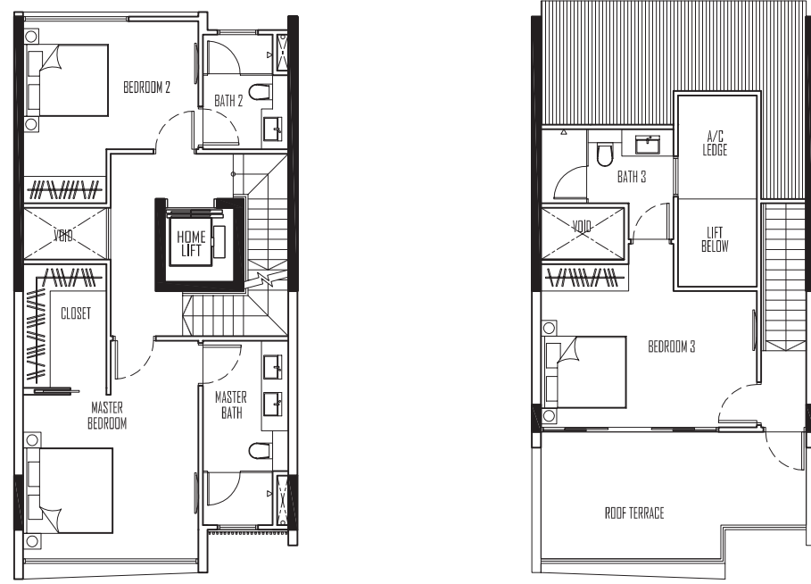
3RD STOREY
