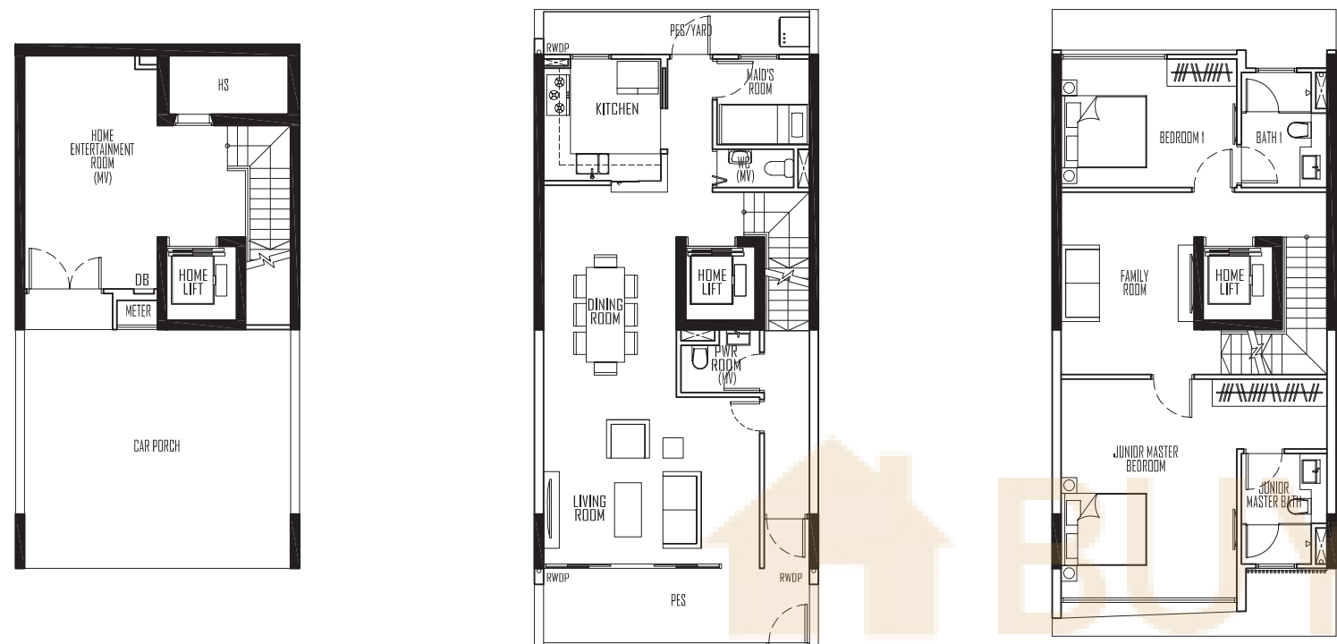
BASEMENT
