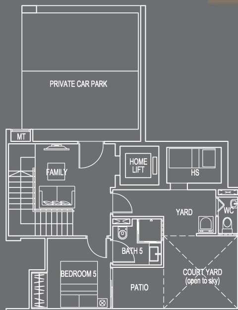
Basement Plan
