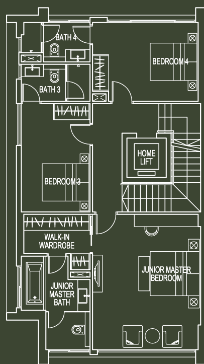
2nd Storey Plan
