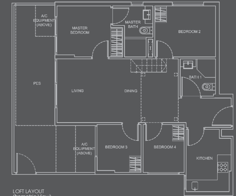
LOFT LAYOUT (Isometric View)
