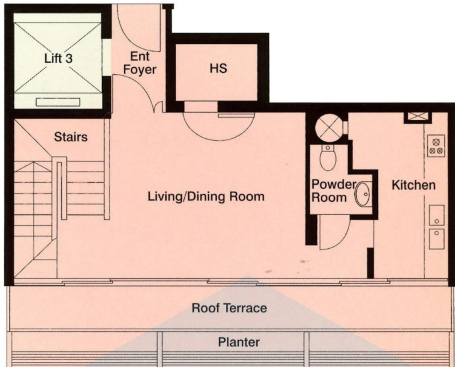
9TH STOREY
