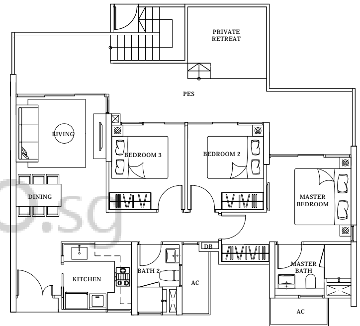
TYPE A1p(r) 115 sq.m. / 1238 sq.ft.
