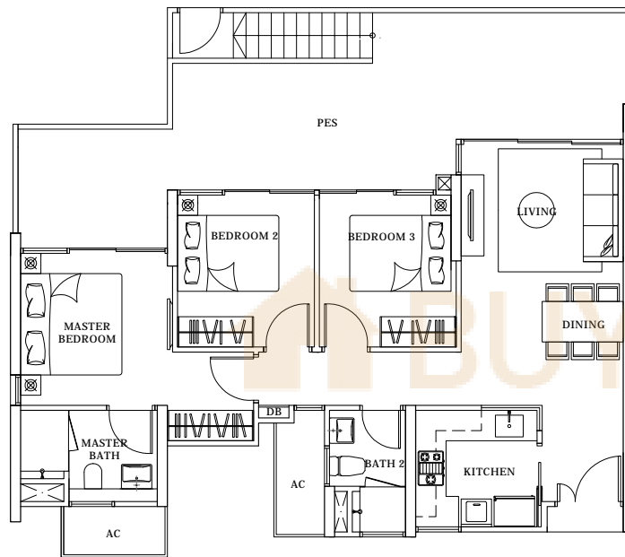
TYPE A1p-1 114 sq.m. / 1227 sq.ft.
