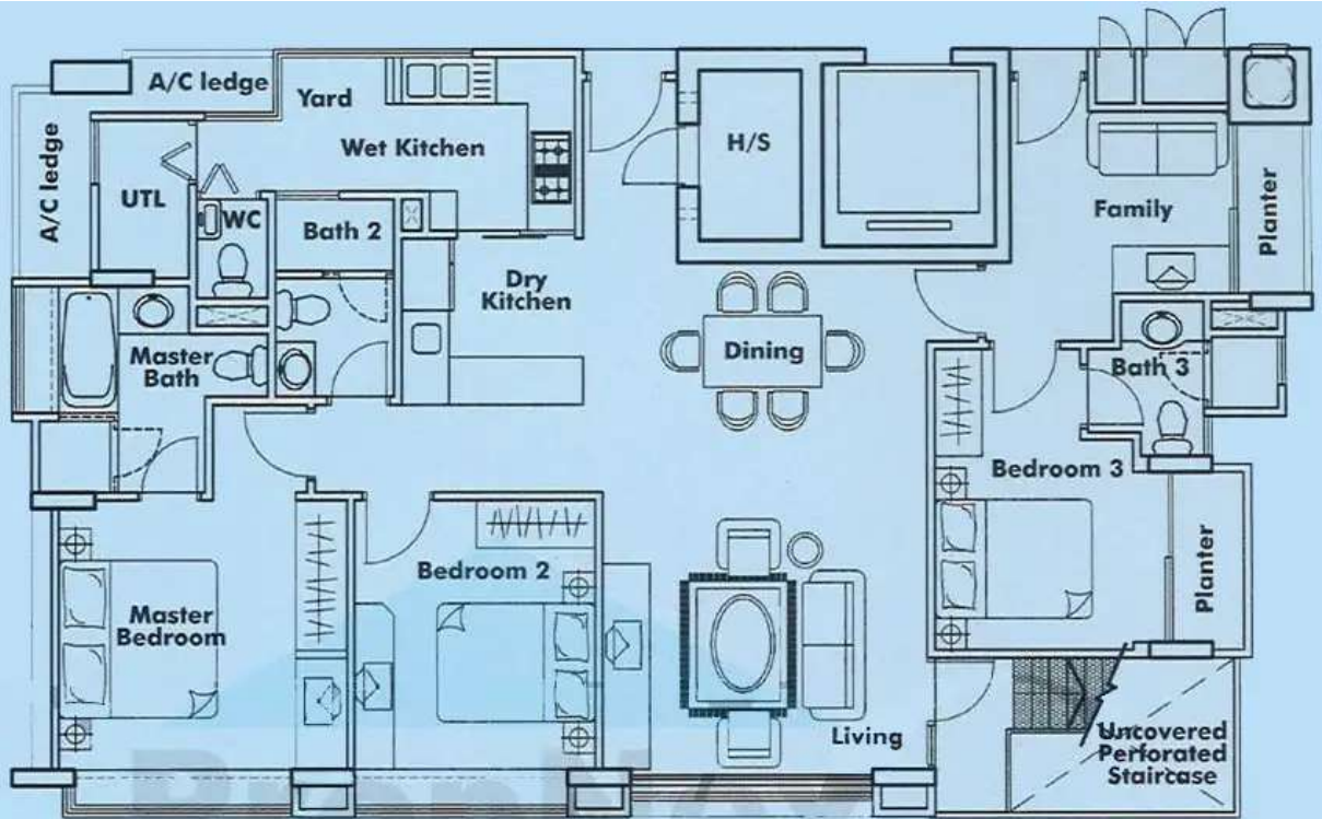
Lower Storey
