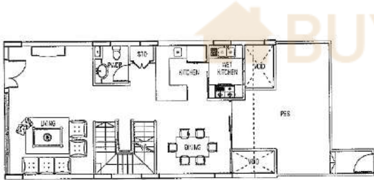
1st Storey
