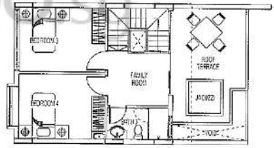
3rd Storey
