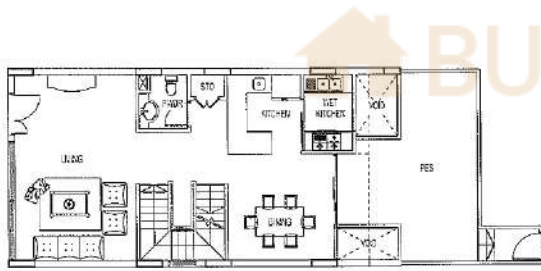
1st Storey
