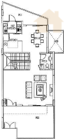
1st Storey
