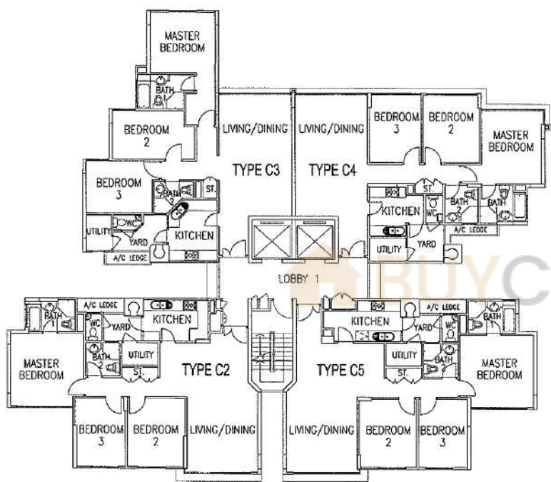
Begonia Tower 1 Geylang East Avenue 1 14th Storey Plan
