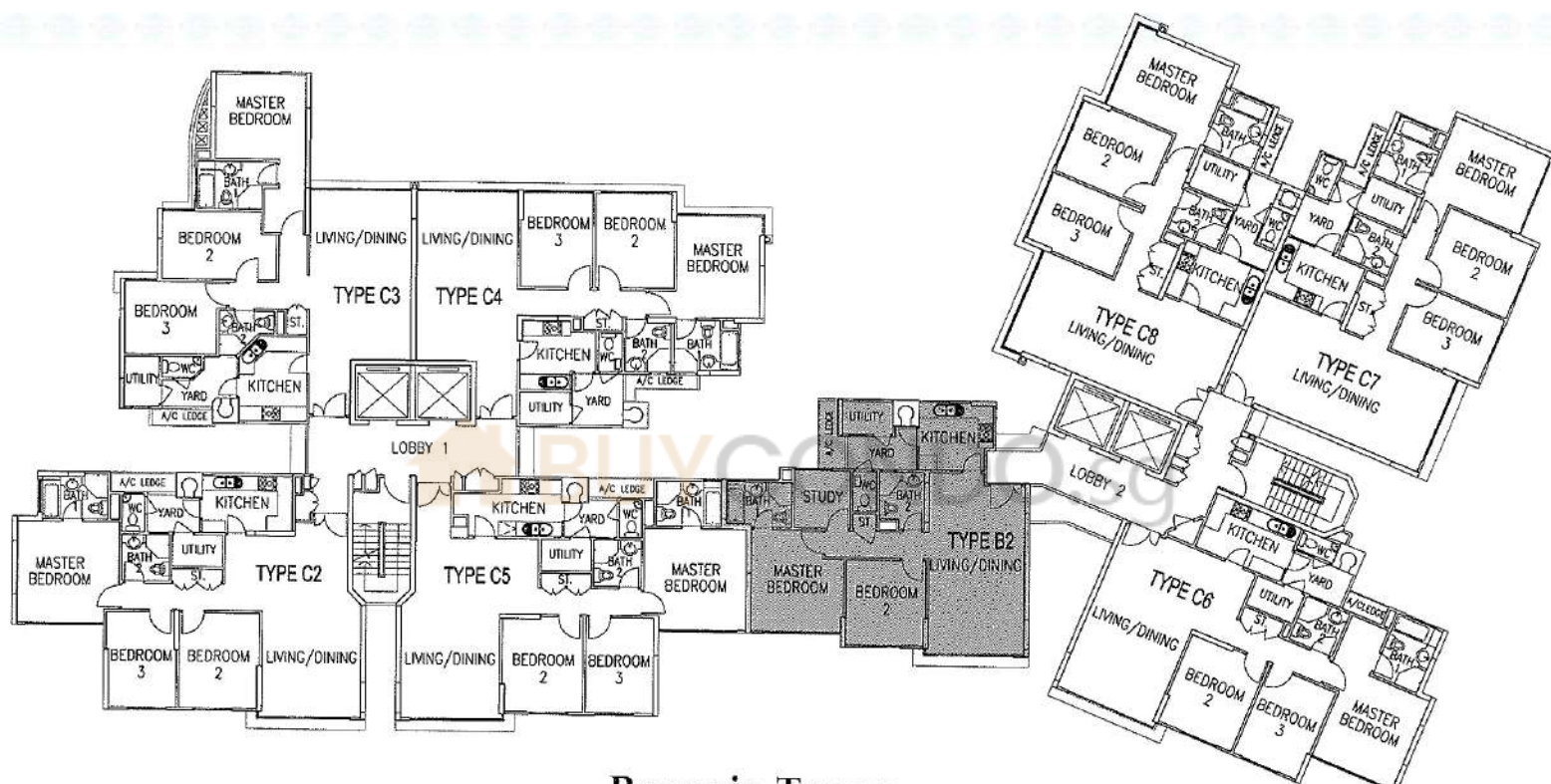
Begonia Tower 1 Geylang East Avenue 1 3rd – 5th Storey Plan
