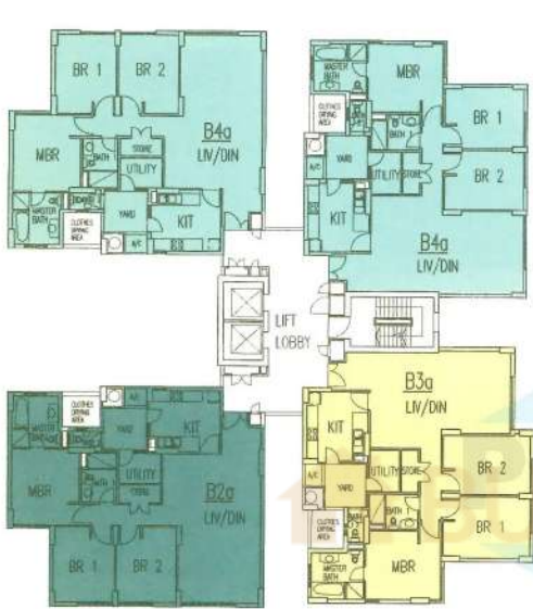
41 Bangkit Rd 5th – 12th Storey Plan
