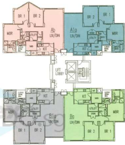
33 Bangkit Rd 15th Storey Plan
