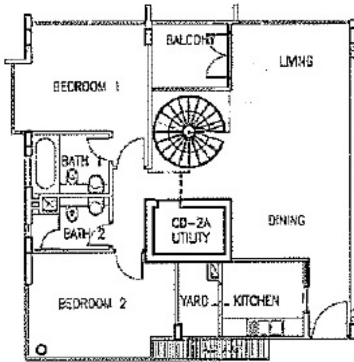
TYPE D1 -with Attic #04-06 (2045sqf)
