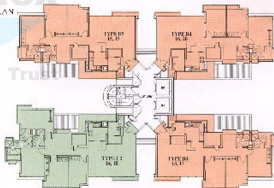
3RD, 6TH, 9TH, 12TH, 15TH & 18TH STOREY PLAN
