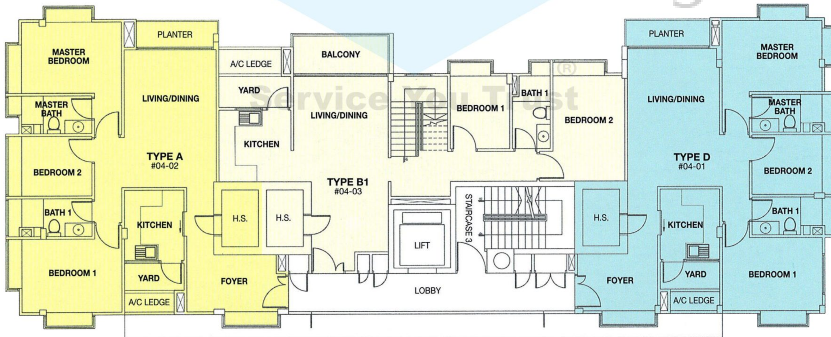
4th Storey
