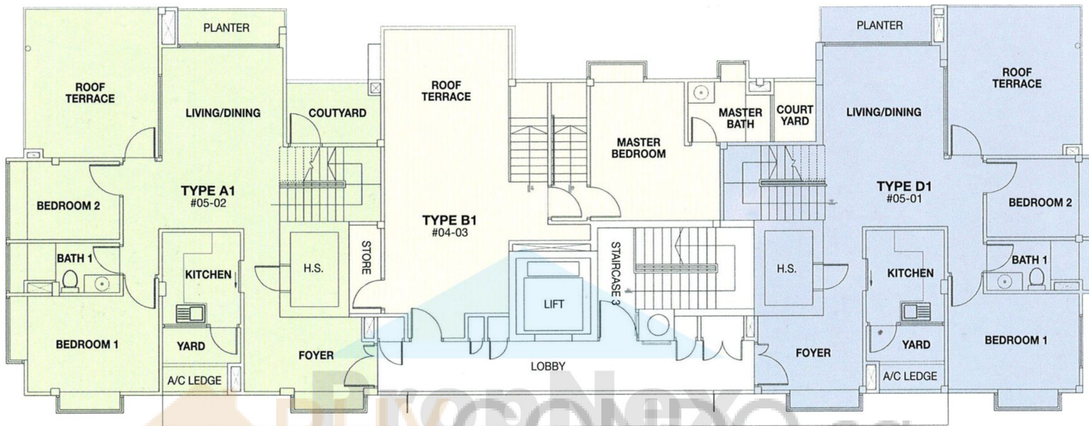
5th Storey
