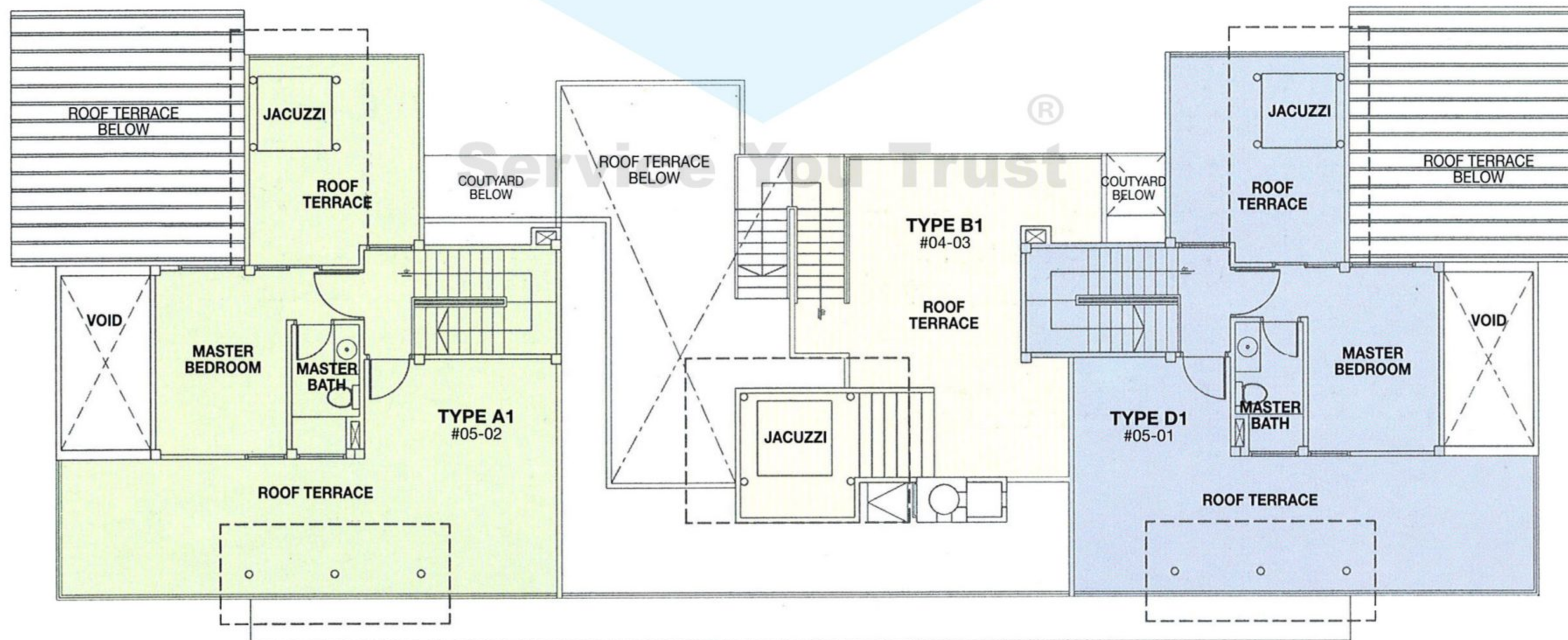
Attic
