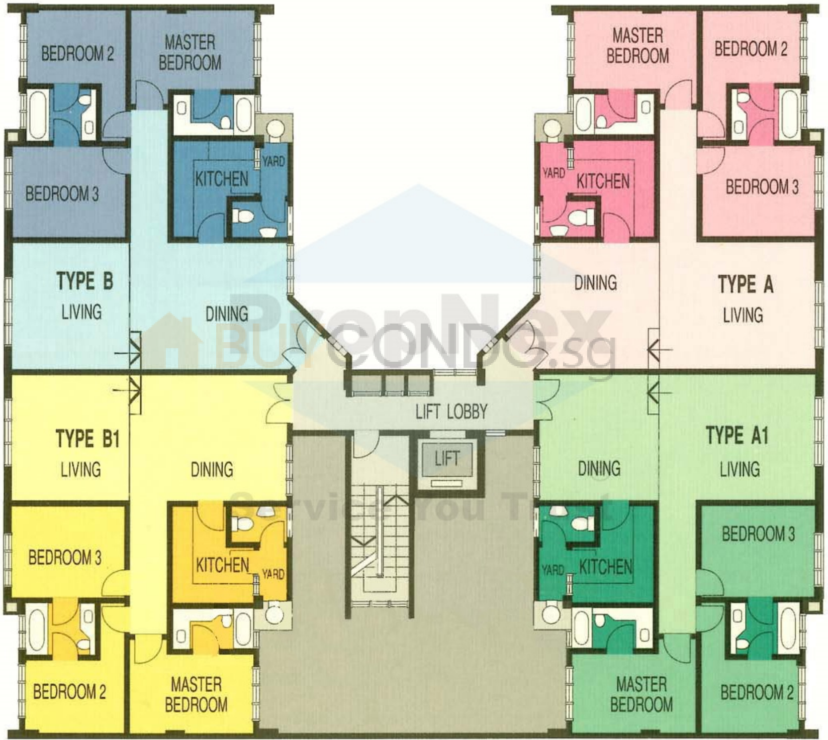
3rd – 8th storey plan
