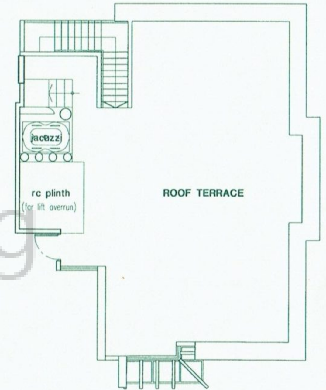
TYPE A1 (Roof Level)
