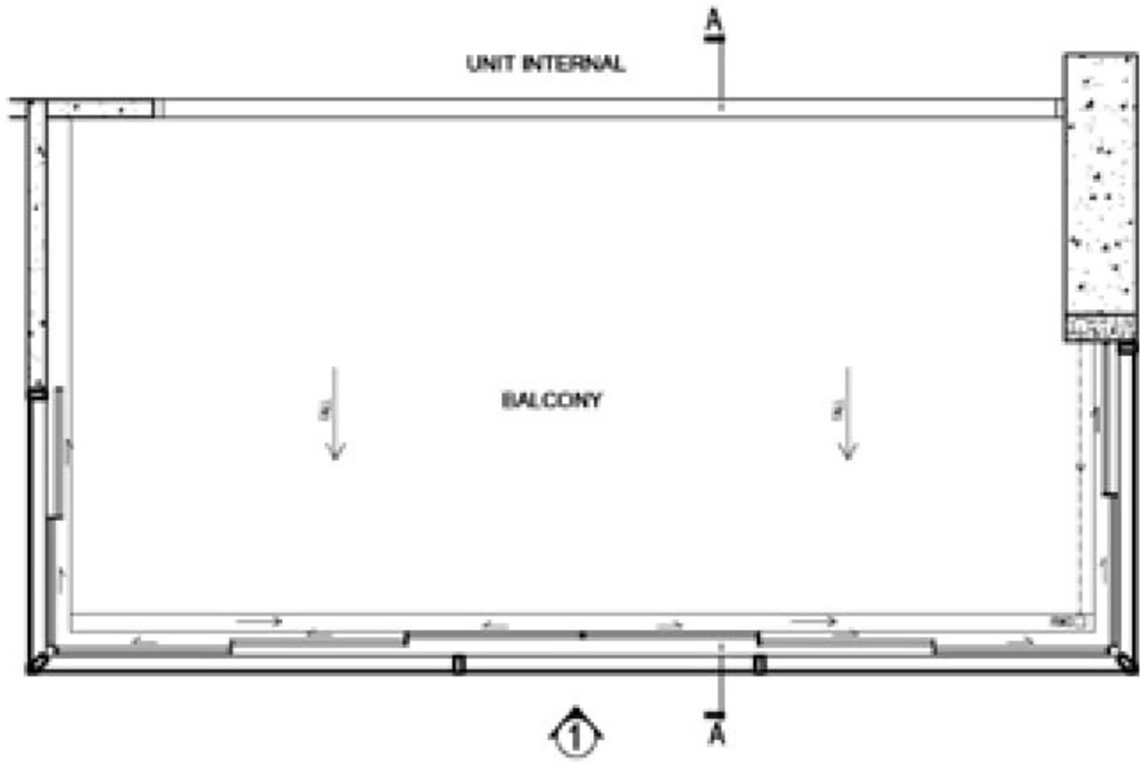
BALCONY SCREEN DETAILS - PART PLAN
