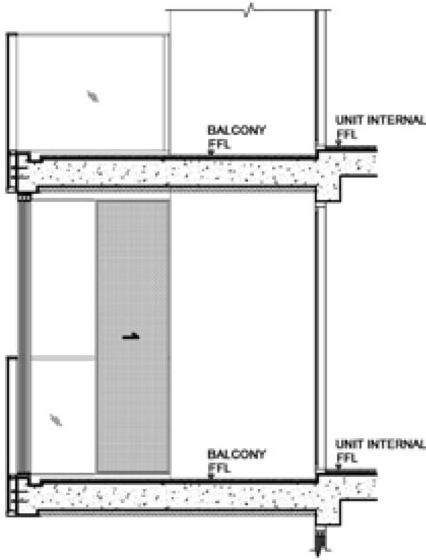
BALCONY DETAILS - SECTION A-A
