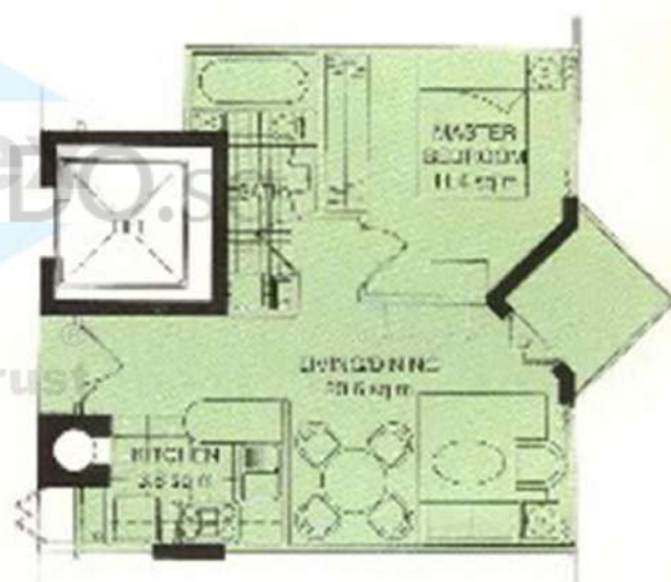
TYPE C 44 sq m (174 sq ft)
