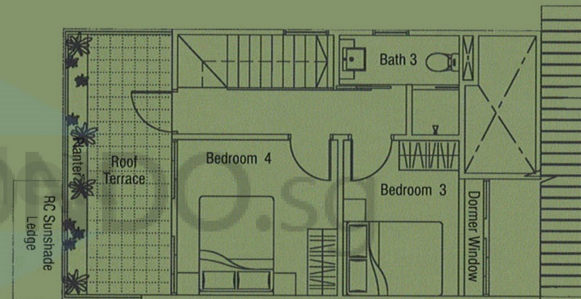
Attic
