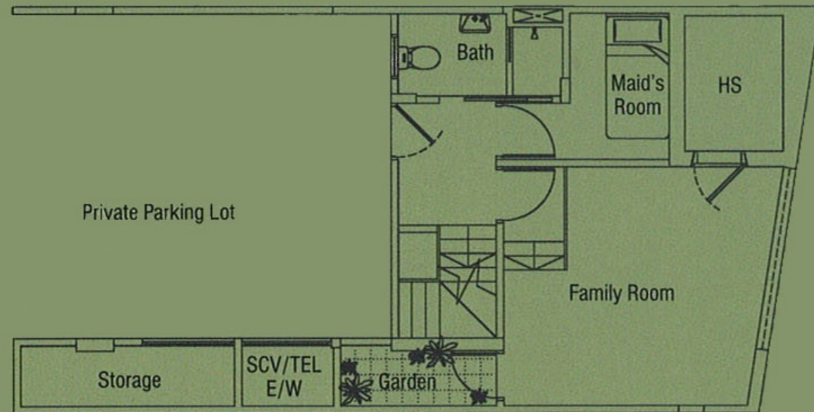
Basement
