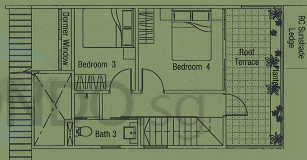
Attic
