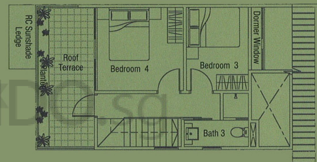
Attic
