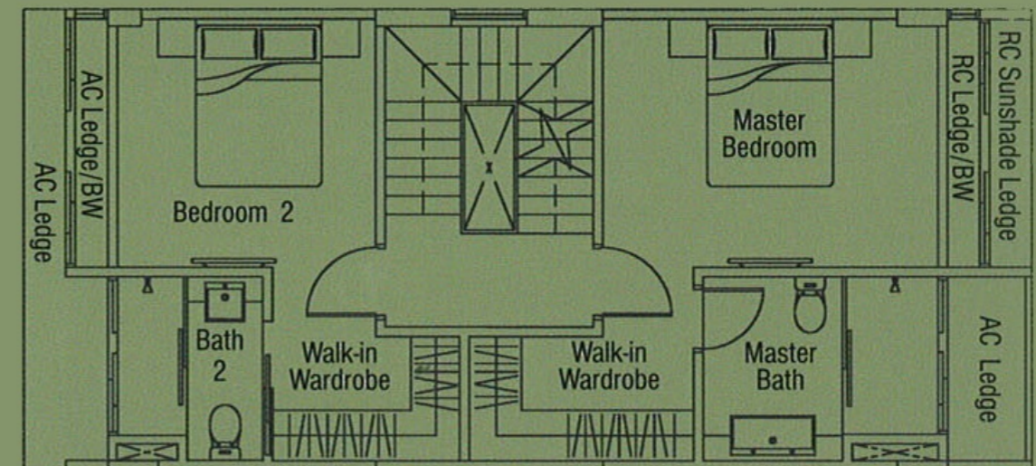
2nd Storey
