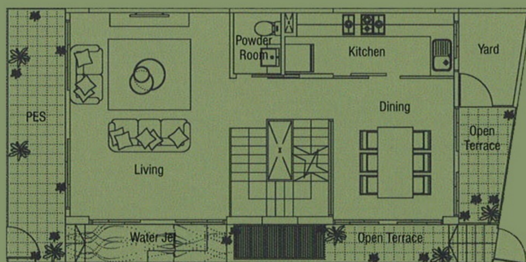
1st Storey
