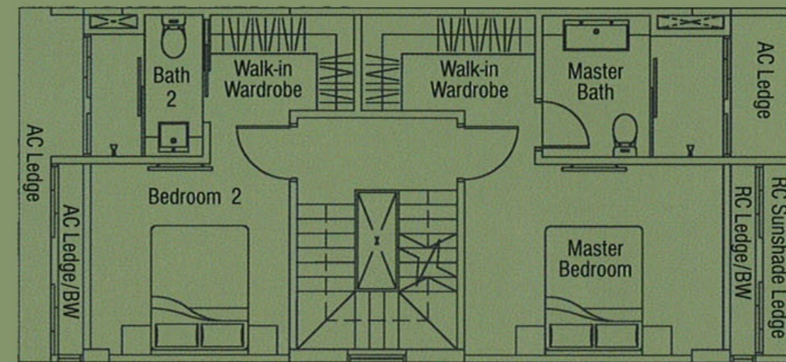
2nd Storey
