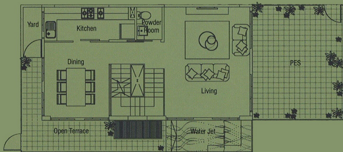
1st Storey
