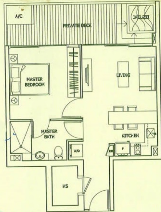
TYPE A4P #01-09 Unit Area 60 sq.m. (646 sq.ft.)
