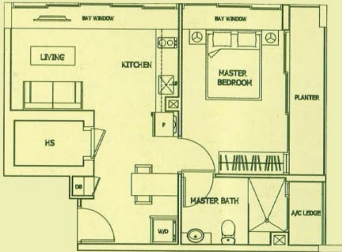
TYPE A3 #02-04 - #04-04 Unit Area 52 sq.m. (560 sq.ft.)
