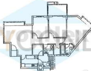
E22 - 181 sqm Living & Dining - 28.66 sqm Master Bedroom - 17.15 sqm Bedroom 1 - 11.91 sqm Bedroom 2 - 10.65 sqm
