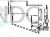
D34 - 59 sqm Living & Dining - 23.78 sqm Master Bedroom - 16.30 sqm
