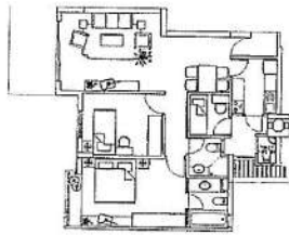
F11 - 88 sqm Living & Dining - 29.26 sqm Master Bedroom - 15.94 sqm Bedroom 1 - 10.36 sqm
