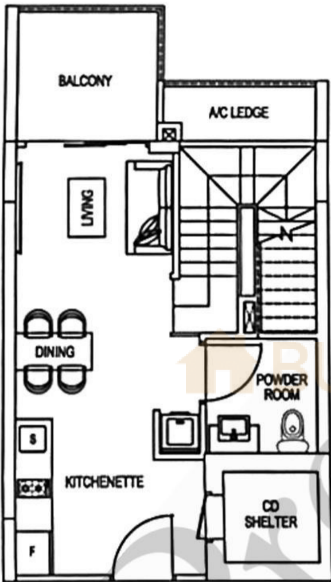
LOWER STOREY
