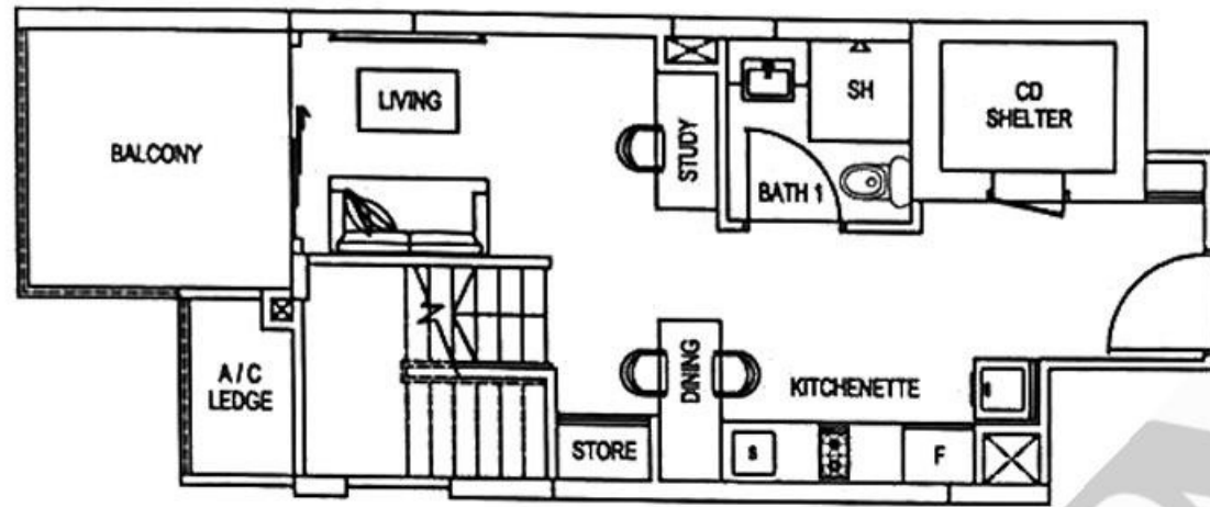
LOWER STOREY
