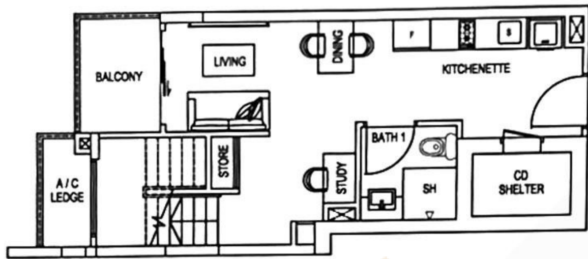
LOWER STOREY
