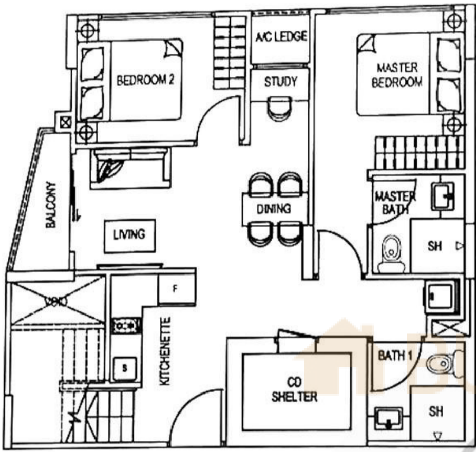
LOWER STOREY
