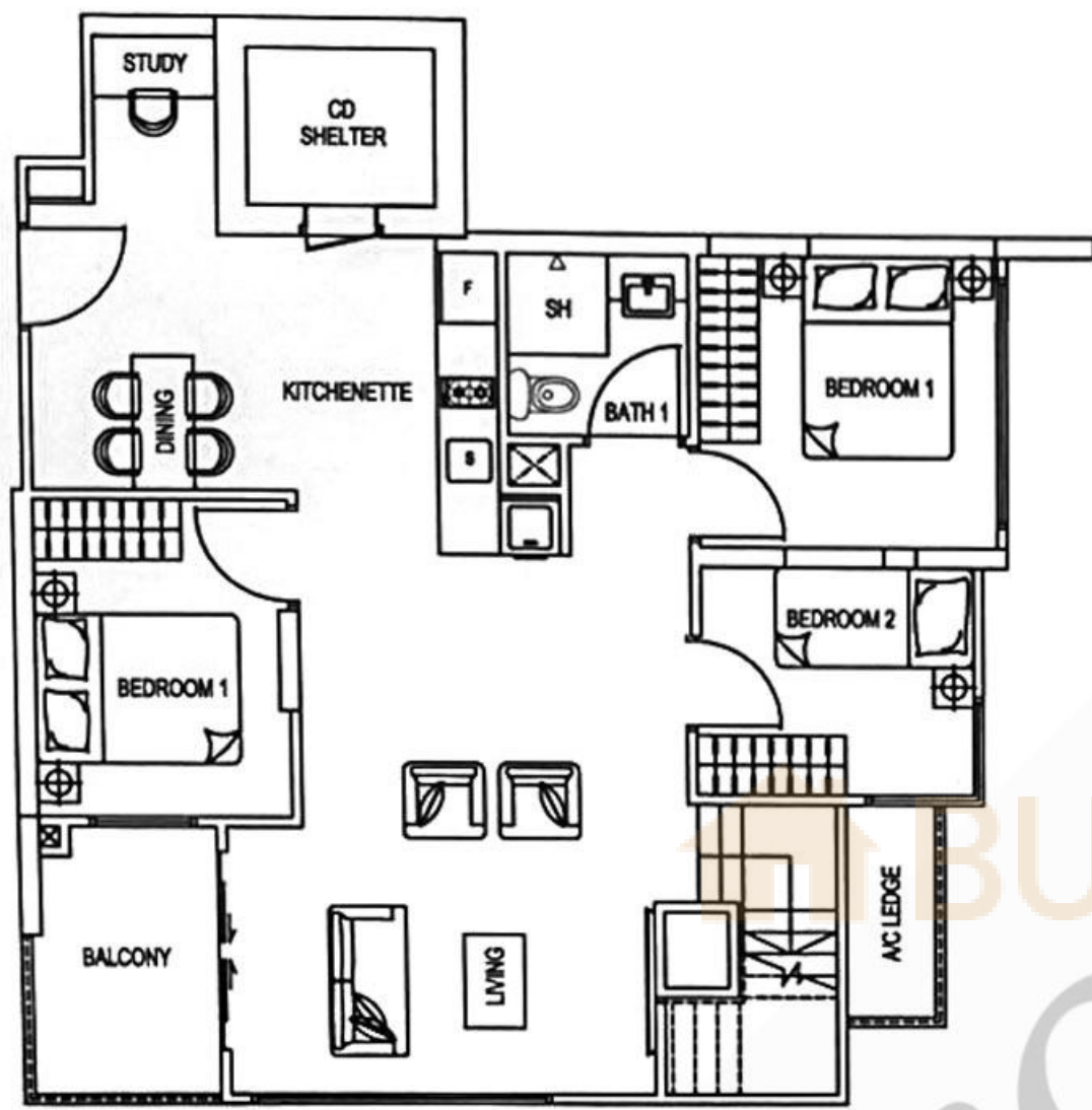
LOWER STOREY
