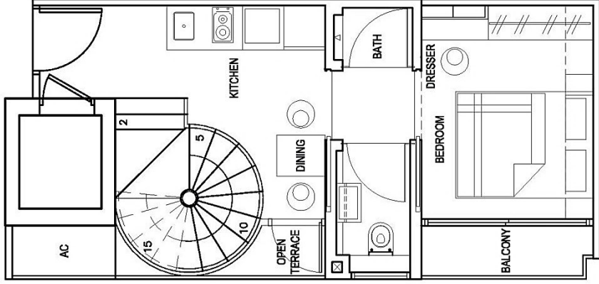
LOWER PENTHOUSE
