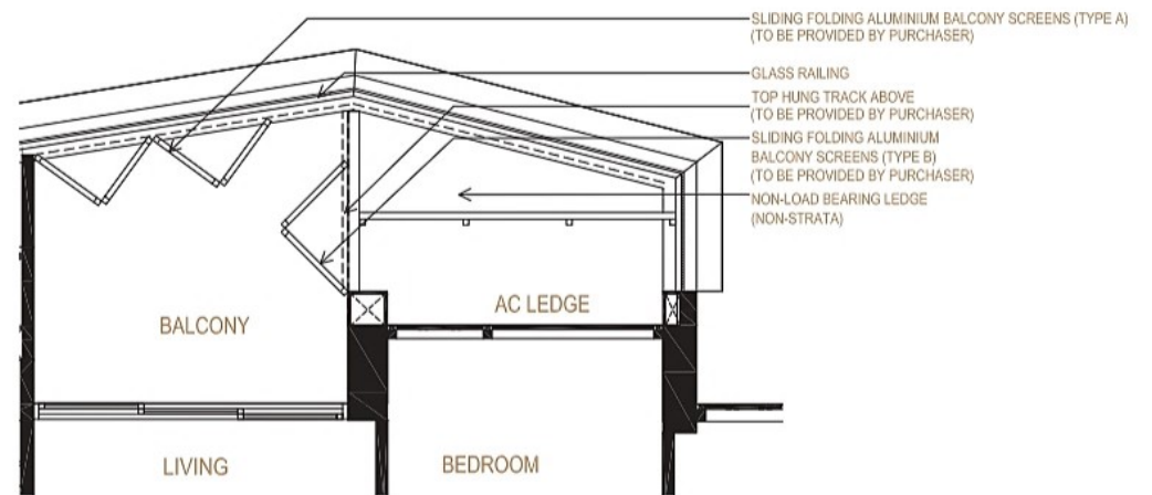
TYPICAL RETRACTABLE BALCONY SCREENING PLAN
