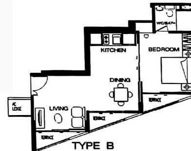
TYPE B #02-01 46 sqm / 495 sqft
