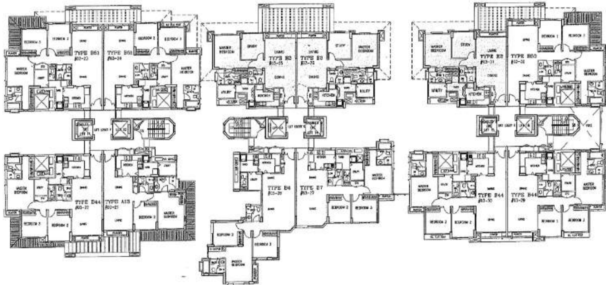
3rd Storey Plan - Block 9
